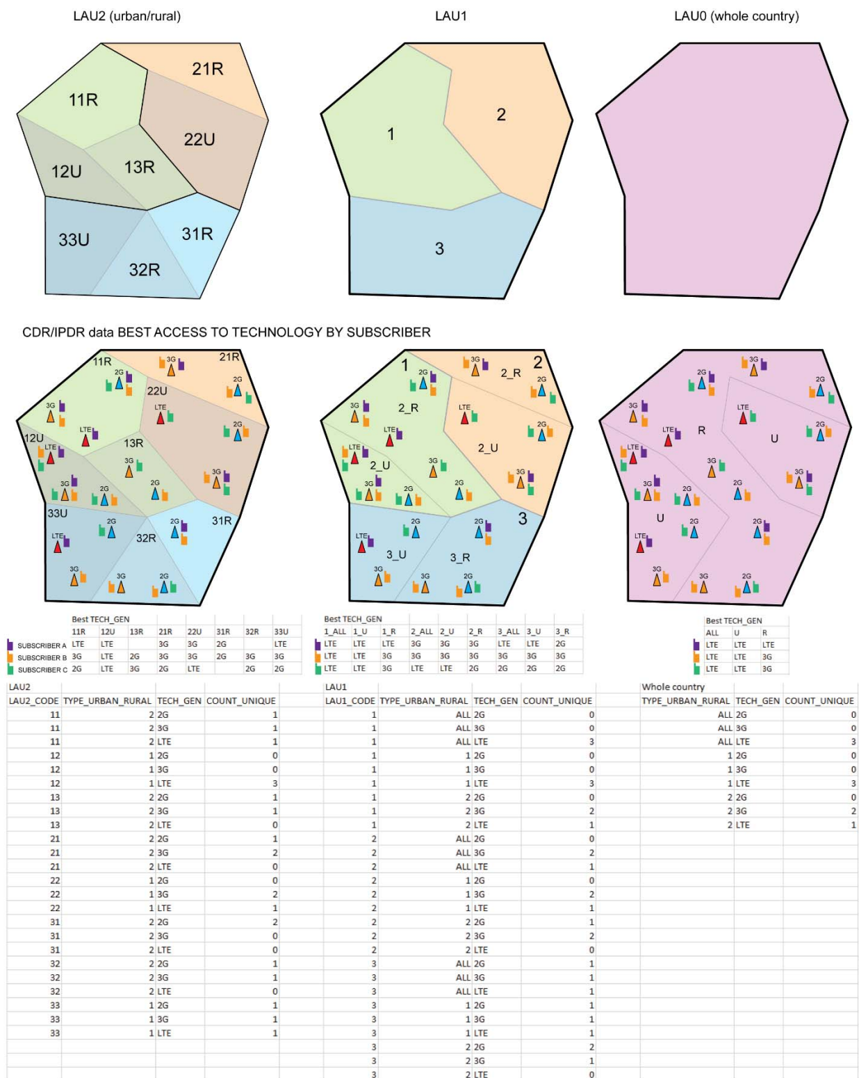
Figure 4. Illustration of assigning the best technology accessed using LAU2, LAU1 and LAU0 levels along with expected results.
